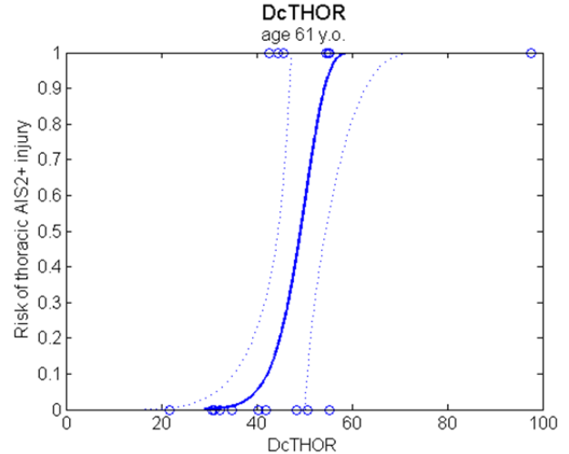
Fig. 7. AIS2+ IRC for DcTHOR and THUMS that were constructed from matched THUMS simulations and PMHS data [9]
