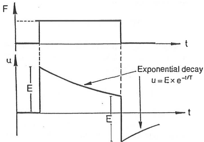
Figure 2. The application of a constant load F to a piezoelectric transducer produces a response u with a decay characterised by a time constant T . The e in the decay formula is the base for natural logarithms \approx 2.718 .
