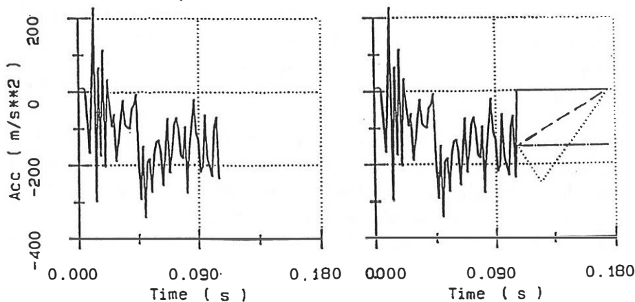
Figure 4. The left diagram shows an impact deceleration pulse. Due to DARR limitations, the recorded pulse is interrupted at 107 ms. The right diagram shows the same pulse, extended with different theoretical tails.
