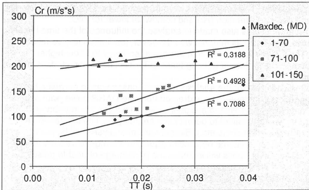
Figure 6. Chest peak resultant acceleration (Cr) vs. triggering time (TT) for different Maximal deceleration levels (MD).
