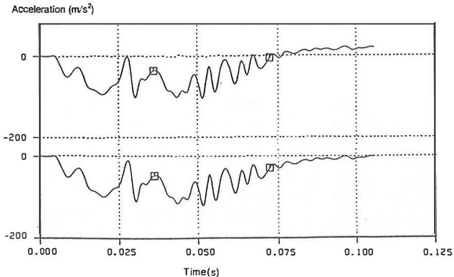
Figure 3. Signals from the DARR accelerometer, before and after correction for the piezoelectric decay.
