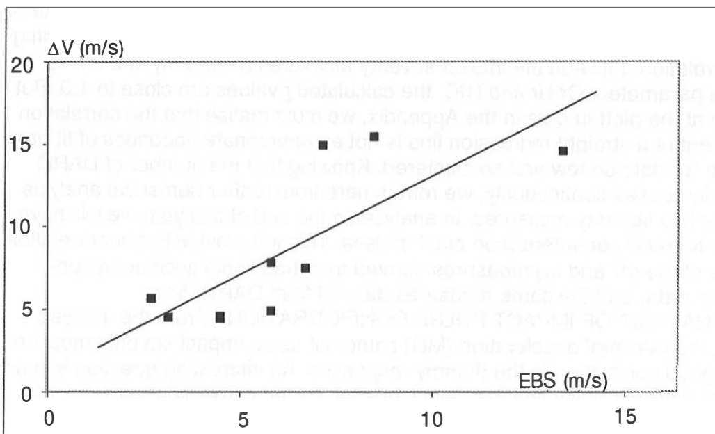
Figure 5. Correlation of \Delta V and EBS, r = 0.79
