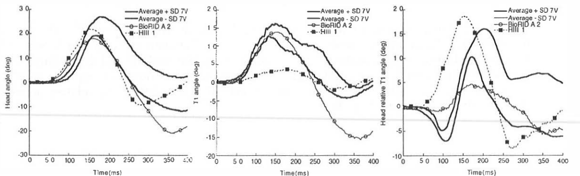
Figure 7: Rearward angular dummy displacements of the head, T1 and head relative to T1 compared to the volunteer response corridors (average \pm standard deviation) at \Delta V=7 km/h.
